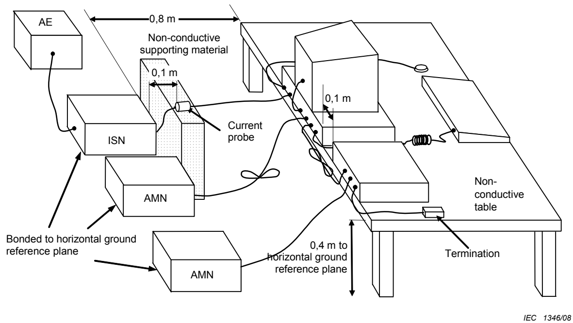
Figure 7 – Example test arrangement for tabletop equipment (conducted emission measurement – alternative 2)
